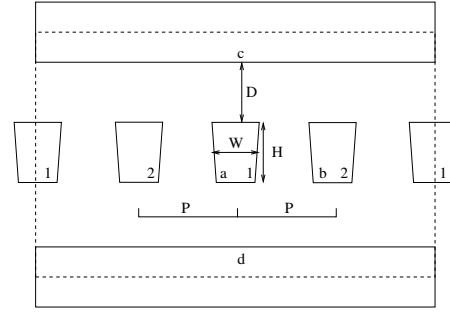
Figure 2: Three interconnect layers shown. Side view. W , H , D and P are the parameters affecting variability in coupling capacitance. Coupling capacitances between interconnect a and interconnects b , c and d are reported in a capacitance table. Interconnects decomposed into mask1 and mask2.
