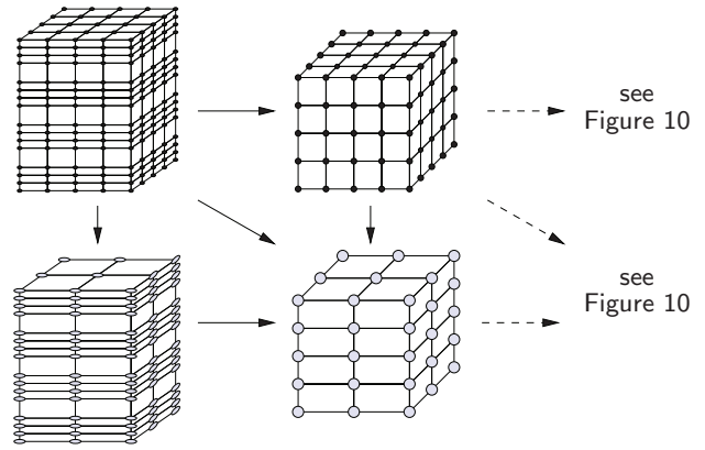
Figure 11: Simplifying the graph of interconnect resources for 3D technologies. From left to right, only layers within a tier are combined resulting in a new (intermediate) simplification step. From top to bottom, simplification is done by combining regions to tiles according to Fig. 10. Further simplification (to the right) is the same as in Fig. 10.
