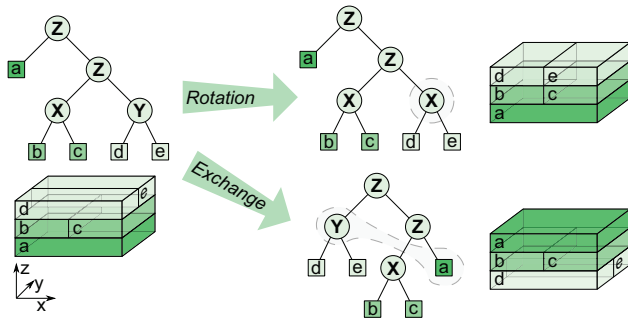
Figure 7: Illustration of 3D Slicing Tree operations to permute a given 3D floorplan. A rotation alters an inner node (representing a cut through the normal plane) resulting in a physical rotation of modules contained in the subtrees of that node. An exchange swaps two subtrees resulting in a physical exchange of modules contained in these subtrees.
