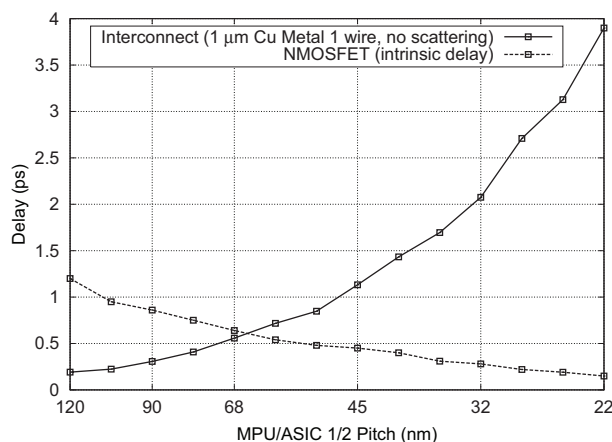
Figure 1: The increasing interconnect delay for various technology nodes according to the ITRS roadmap [1].
