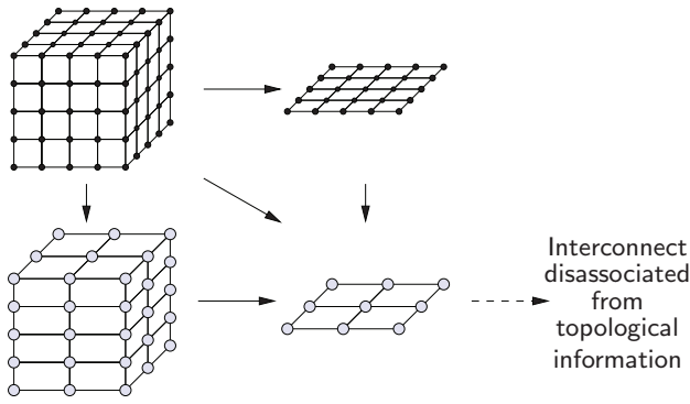
Figure 10: Simplifying the graph of interconnect resources for 2D technologies. From left to right, the number of interconnect layers that are treated separately is reduced. From top to bottom, regions within a layer are combined to tiles and treated as an atomic unit. Further reduction would remove any information about layout topology, leading to prediction methods such as complexity analysis [22] and Rent’s rule [21].
