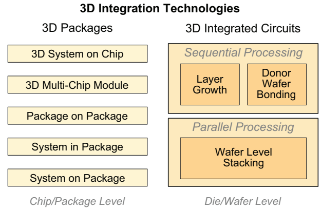
Figure 2: Today's most common 3D integration technologies. 3D packages enable functional systems on a higher system level. 3D integrated circuits utilize wafer level integration to achieve high inter-layer interconnect densities.
