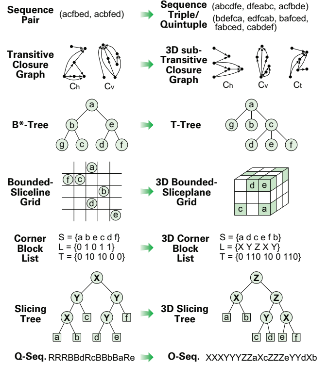
Figure 6: Classical 2D floorplanning data structures (left) and their 3D counterparts (right, see also Table 2).
