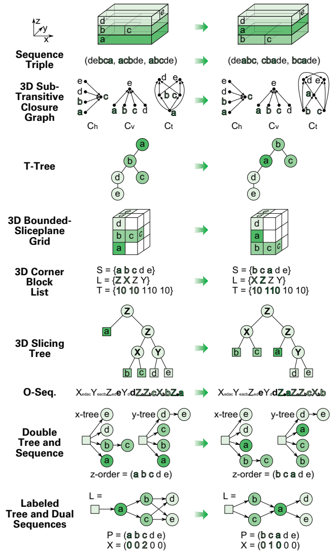
Figure 8: 3D block swapping example using new 3D data structures. As illustrated at the top, block a is exchanged with blocks ( b , c ).
