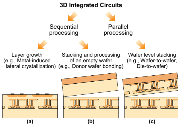
Figure 4: Classification of 3D ICs with regard to their technology. While layer growth (a) and donor wafer bonding (b) require a sequential processing of the various device layers, wafer level stacking (c) enables a parallel fabrication of these layers.
