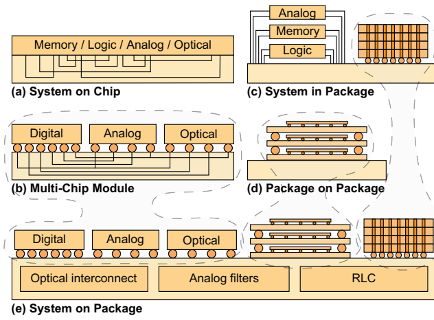
Figure 3: Modern 3D packages and their relation with each other.
