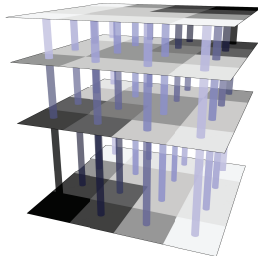
Figure 13: 3D interconnect and TSV density predicted analogously to Lou's model for a two terminal net routed in four tiers. The pins of the net are at the bottom left corner and at the top right corner. Black squares denote the highest interconnect density, white denotes the lowest density. The predicted TSV density is illustrated by colored columns. Dark columns indicate a high TSV density, light columns indicate a low density.
